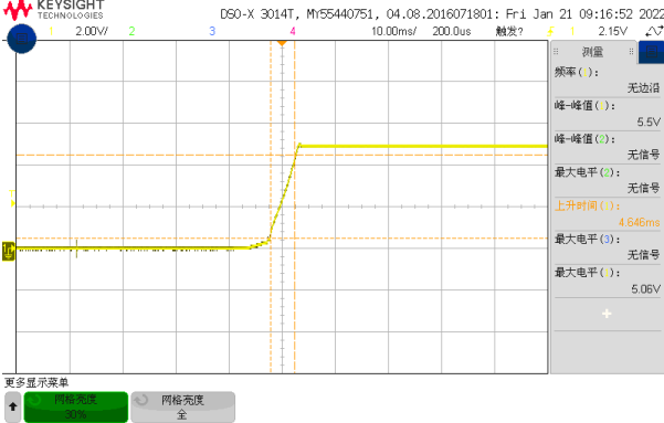
Figure 5, Output voltage established (Iout = 20A)
