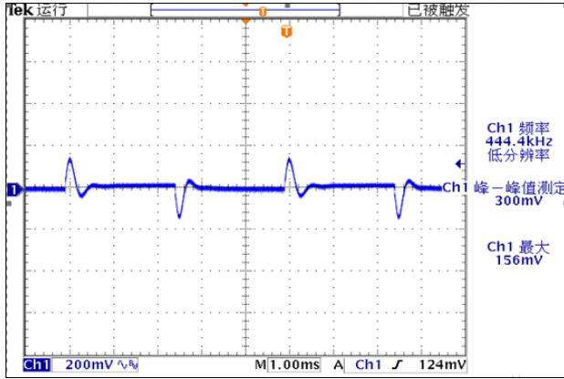
Figure 4, 25% - 50% load dynamic
