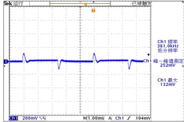
Figure 5, 50% - 75% load dynamic
