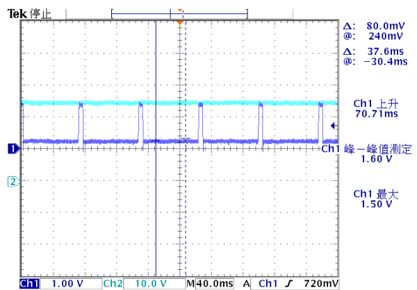
Figure 9, Short-circuit & Output voltage (Iout = 100A)
