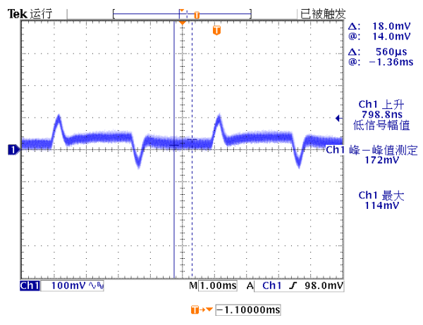
Figure 5, 50% - 75% load dynamic
