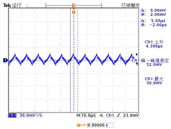
Figure 7, Output ripple & noise (Iout = 100A)
