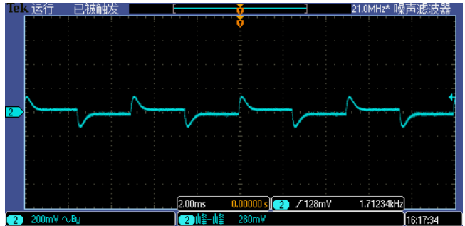
Figure 5, 50% - 75% load dynamic
