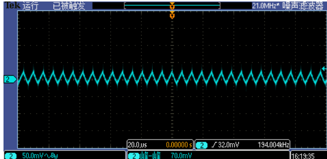
Figure 7, Output ripple & noise (Iout = 30A)
