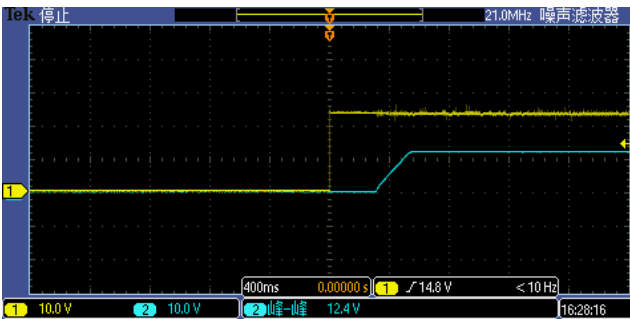
Figure 6, Output voltage established (Iout = 30A)
