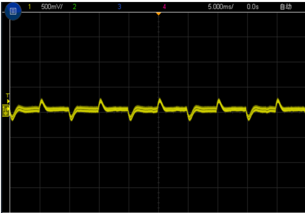
Figure 4, 25% - 50% load dynamic
