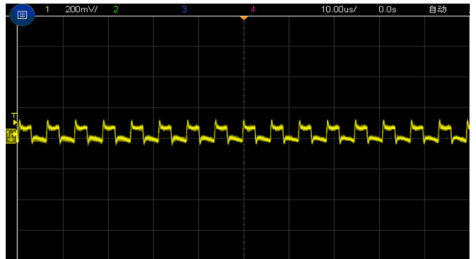
Figure 7, Output ripple & noise (Iout = 15A)
