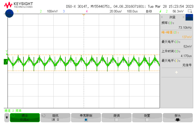
Figure 7, Output ripple & noise (Iout = 85A)
