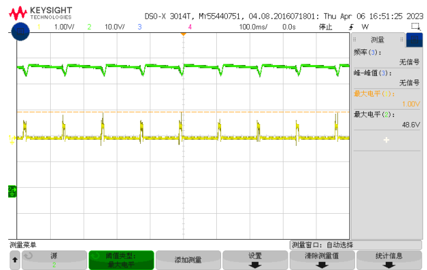
Figure 9, Short-circuit & Output voltage (Iout = 85A)
