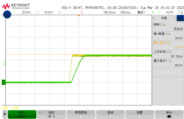
Figure 8, Boot delay time (Iout = 85A)
