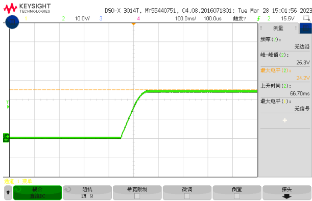
Figure 6, Output voltage established (Iout = 85A)
