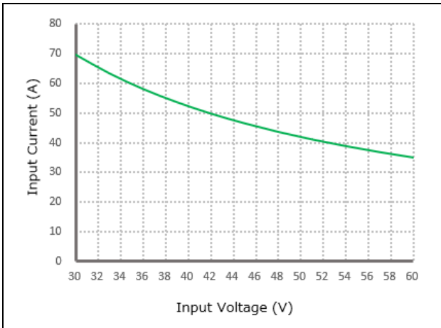
Figure 3, Input V-I, Iout=85A
