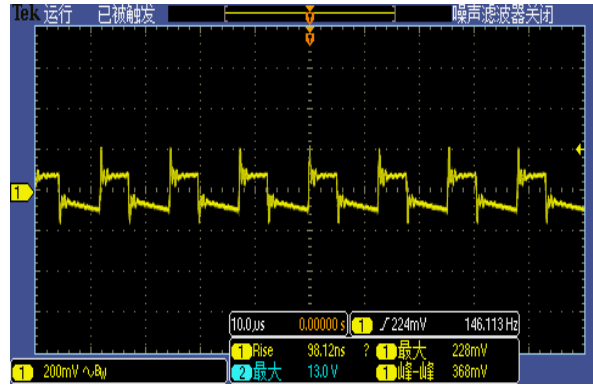
Figure 7, Output ripple & noise (Iout = 25A)
