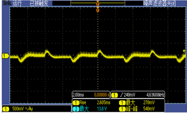
Figure 4, 25% - 50% load dynamic
