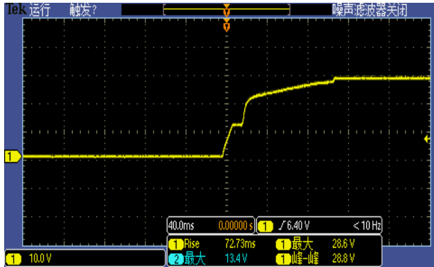
Figure 6, Output voltage established (Iout = 25A)
