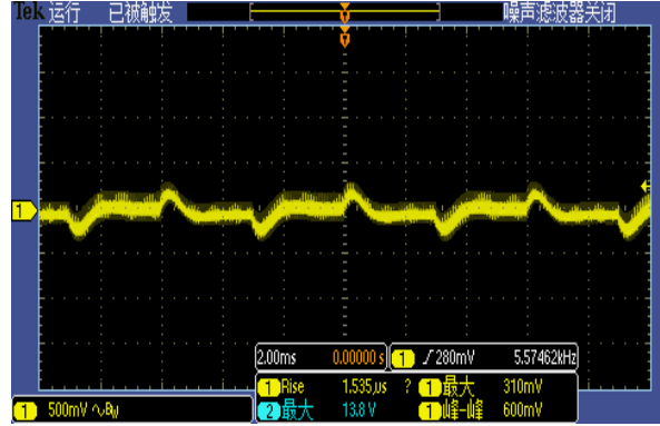
Figure 5, 50% - 75% load dynamic
