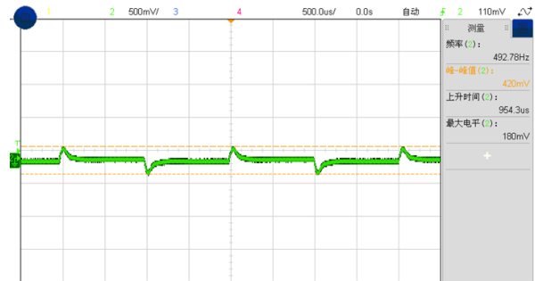
Figure 5, 50% - 75% load dynamic
