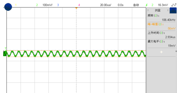
Figure 7, Output ripple & noise (Iout = 30A)
