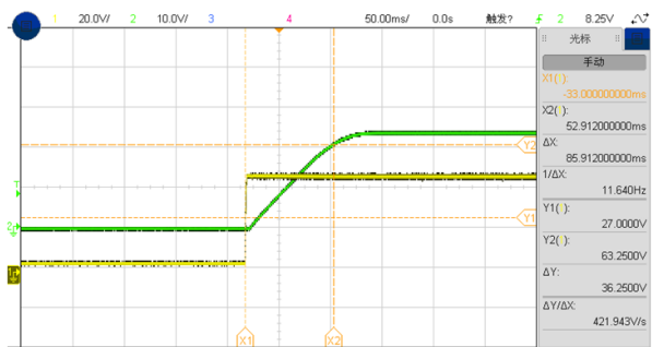
Figure 8, Boot delay time (Iout = 30A)
