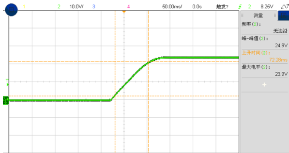
Figure 6, Output voltage established (Iout = 30A)
