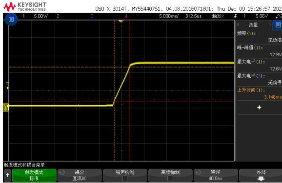
Figure 6, Output voltage established (Iout = 3A)
