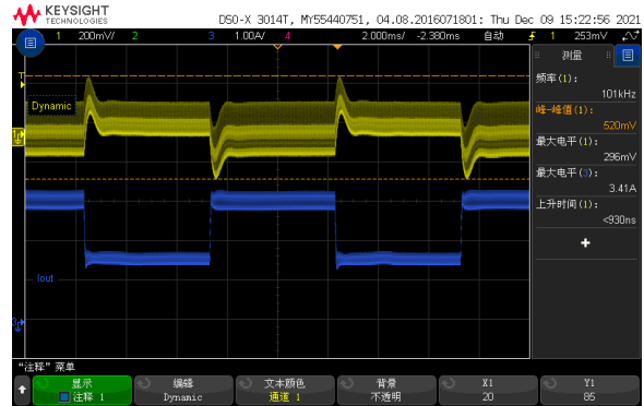
Figure 5, 50% - 75% load dynamic
