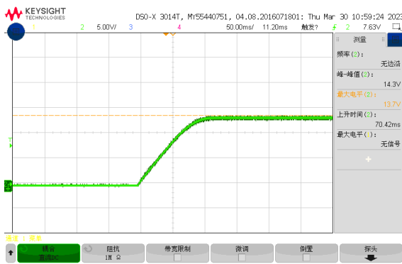
Figure 6, Output voltage established (Iout = 40A)
