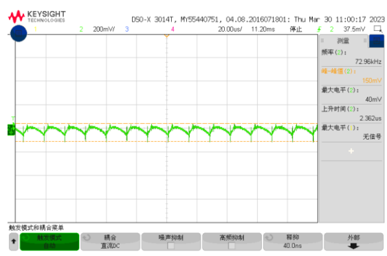
Figure 7, Output ripple & noise (Iout = 40A)
