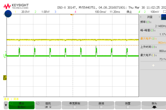
Figure 9, Short-circuit & Output voltage (Iout = 40A)
