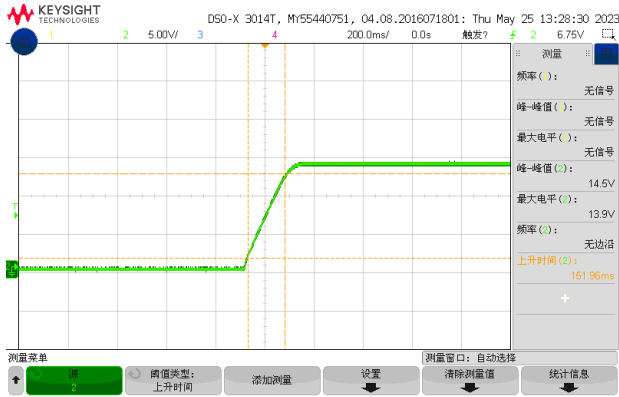
Figure 6, Output voltage established (Iout = 30A)
