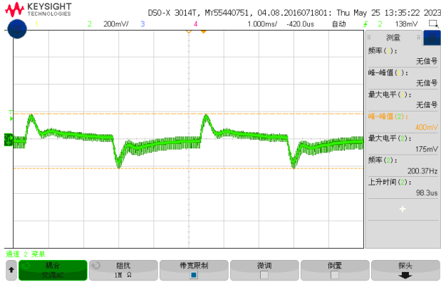
Figure 4, 25% - 50% load dynamic
