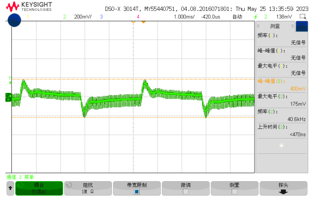
Figure 5, 50% - 75% load dynamic
