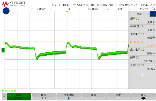
Figure 4, 25% - 50% load dynamic
