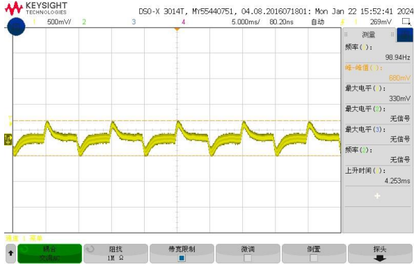
Figure 4, 25% - 50% load dynamic
