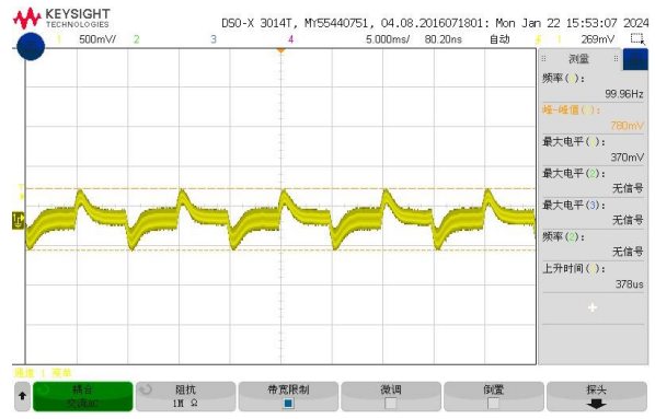
Figure 5, 50% - 75% load dynamic
