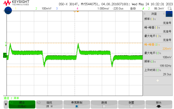
Figure 5, 50% - 75% load dynamic
