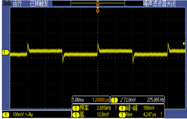
Figure 4, 25% - 50% load dynamic
