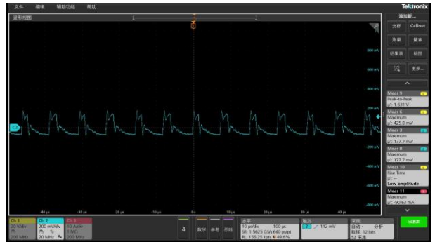
Figure 7, Output ripple & noise (Iout = 15A)
