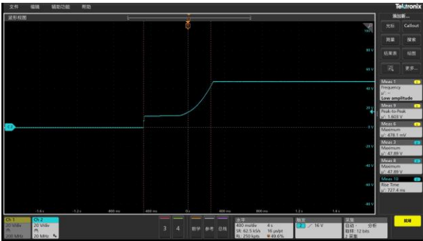
Figure 6, Output voltage established (Iout = 15A)
