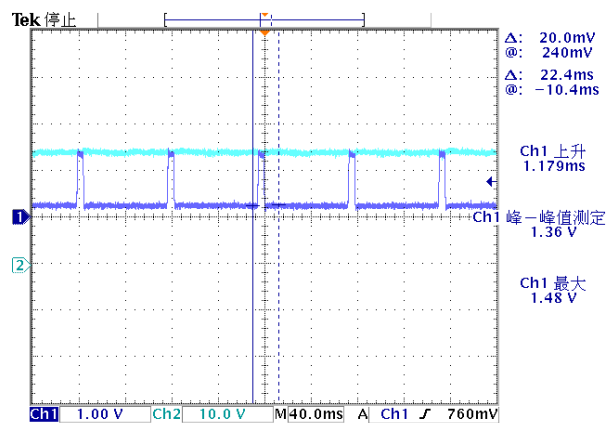
Figure 9, Short-circuit & Output voltage (Iout = 85A)
