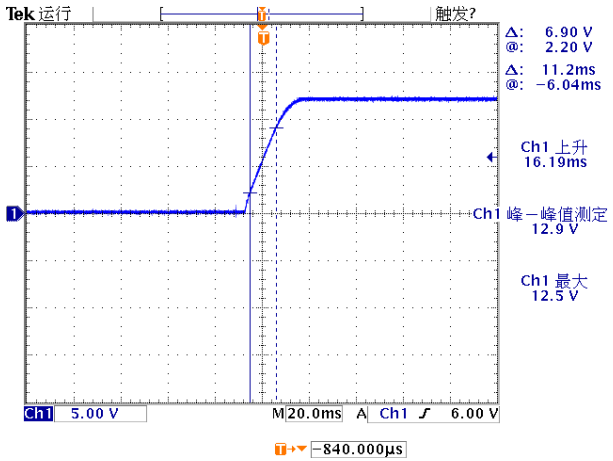
Figure 6, Output voltage established (Iout = 85A)
