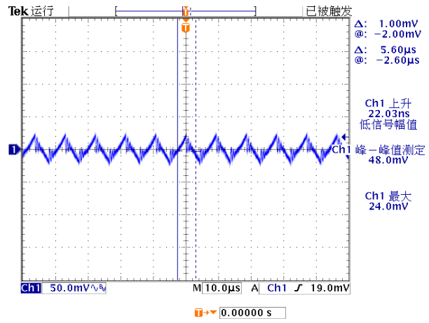
Figure 7, Output ripple & noise (Iout = 85A)
