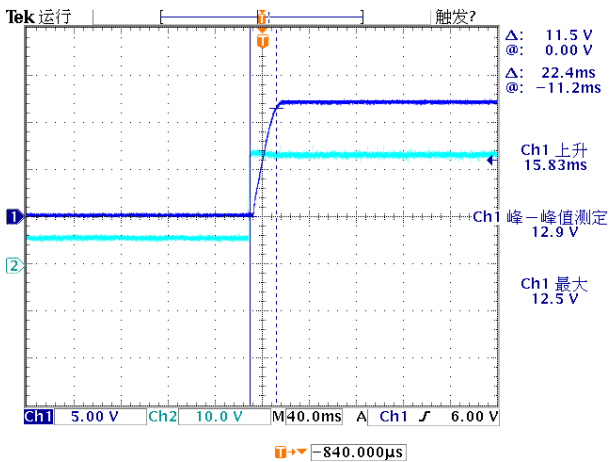
Figure 8, Boot delay time (Iout = 85A)
