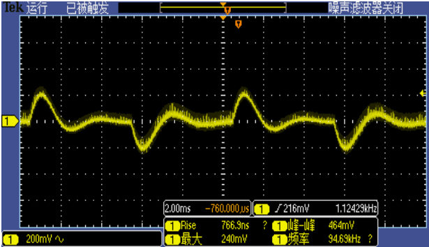
Figure 4, 25% - 50% load dynamic
