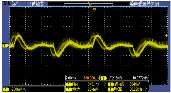
Figure 5, 50% - 75% load dynamic
