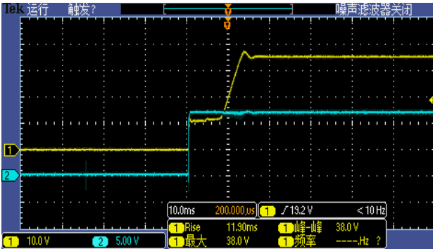
Figure 6, Output voltage established (Iout = 2A)
