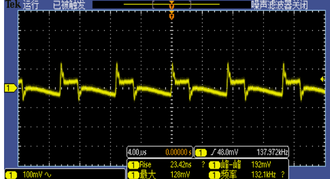
Figure 7, Output ripple & noise (Iout = 2A)
