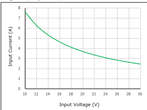
Figure 3, Input V-I, Iout=2A
