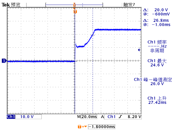
Figure 6, Output voltage established (Iout = 30A)
