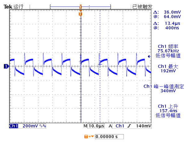
Figure 7, Output ripple & noise (Iout = 30A)
