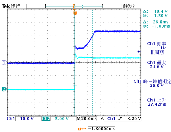
Figure 8, Boot delay time (Iout = 30A)
