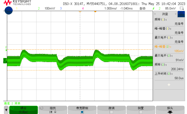
Figure 5, 50% - 75% load dynamic
