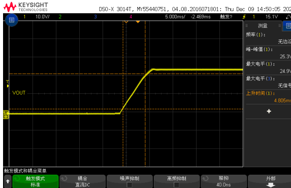
Figure 6, Output voltage established (Iout = 2A)
