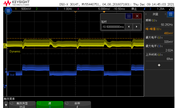
Figure 5, 50% - 75% load dynamic
