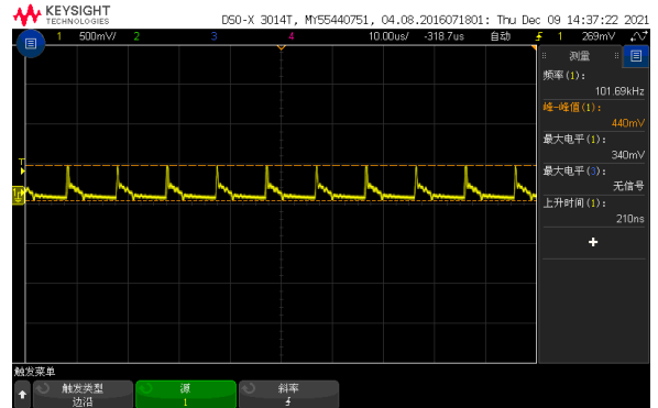
Figure 7, Output ripple & noise (Iout = 2A)
