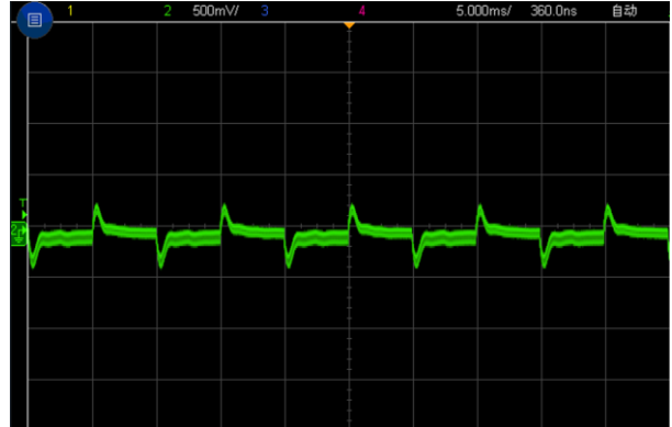
Figure 5, 50% - 75% load dynamic
