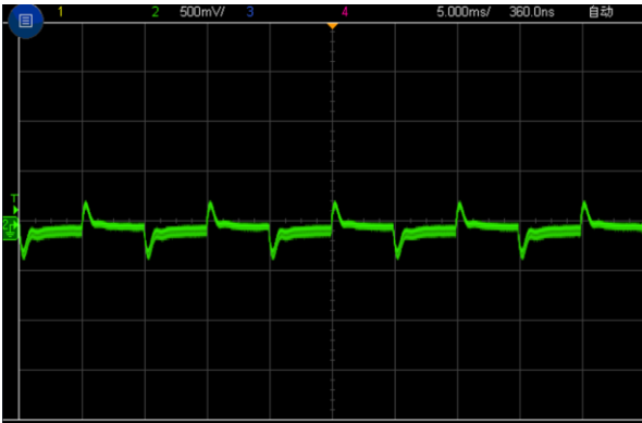
Figure 4, 25% - 50% load dynamic
