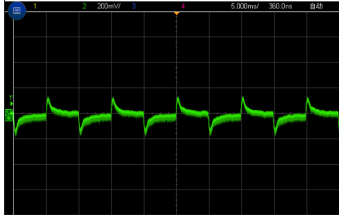
Figure 5, 50% - 75% load dynamic
