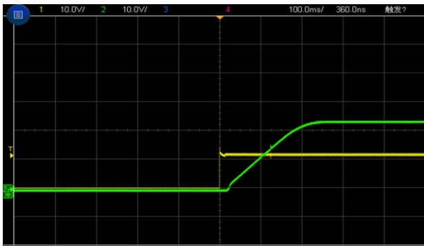
Figure 6, Output voltage established (Iout = 10A)
