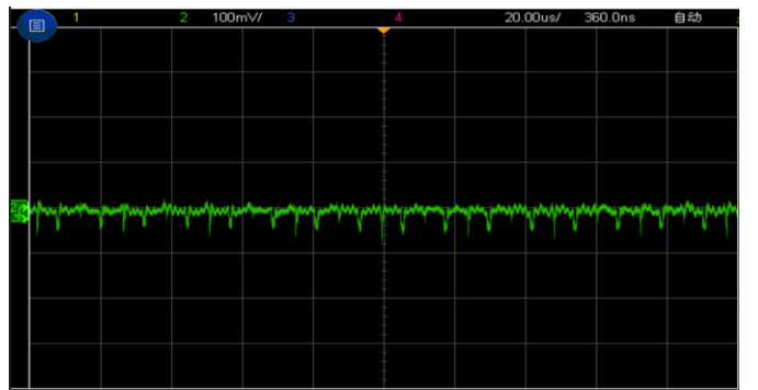
Figure 7, Output ripple & noise (Iout = 10A)
