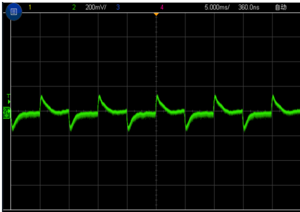
Figure 4, 25% - 50% load dynamic
