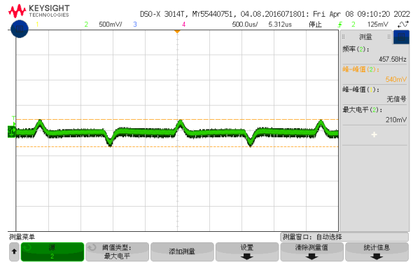
Figure 5, 50% - 75% load dynamic
