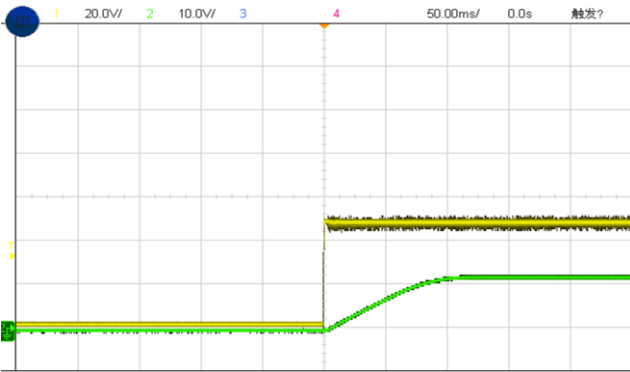
Figure 6, Output voltage established (Iout = 10A)
