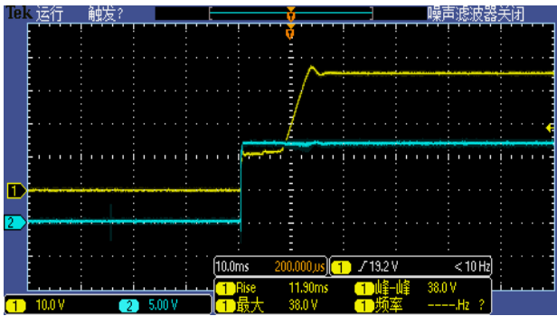
Figure 6, Output voltage established (Iout = 1A)
