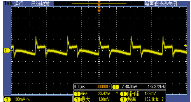
Figure 7, Output ripple & noise (Iout = 1A)
