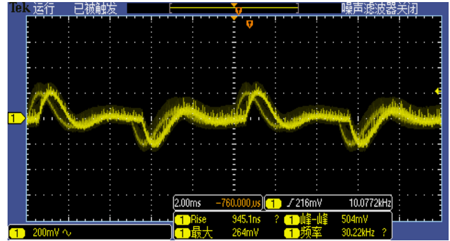
Figure 5, 50% - 75% load dynamic
