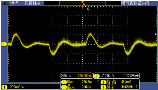
Figure 4, 25% - 50% load dynamic
