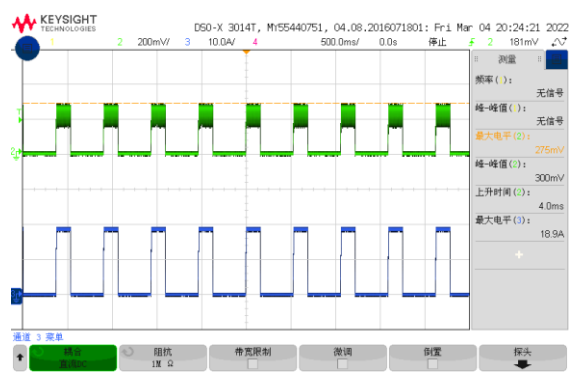
Figure 9, Short circuit & Output voltage
