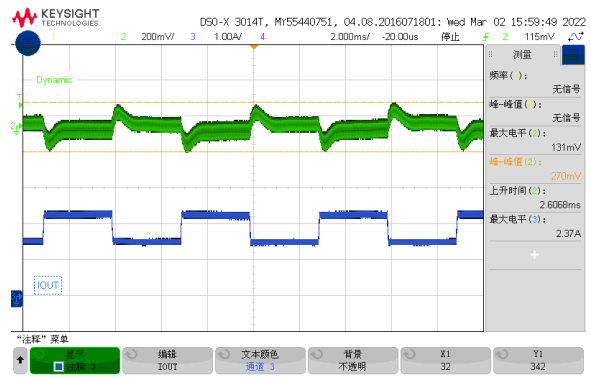
Figure 5, 50% - 75% load dynamic
