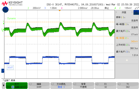
Figure 4, 25% - 50% load dynamic
