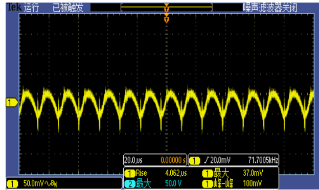
Figure 7, Output ripple & noise (Iout = 60A)
